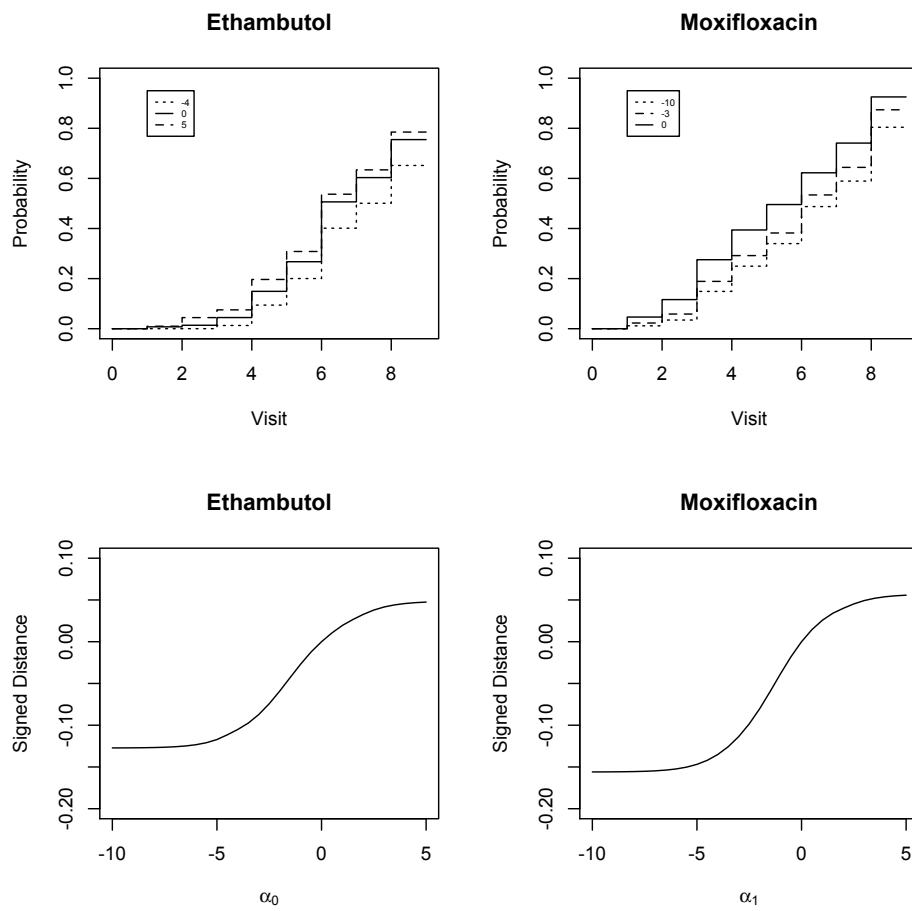
FIG 4. First Row: Treatment-specific estimated distribution of time of culture conversion for the benchmark ( \alpha_0 = 0, \alpha_1 = 0 ) and alternative ( \alpha_0 = 5.0, \alpha_1 = -3 ) sensitivity-analysis parameters. Second Row: For each treatment group, the signed Kolmogorov distance between the estimated distribution of time of culture conversion for given \alpha and the estimated distribution function of time of culture conversion under the benchmark assumption.
