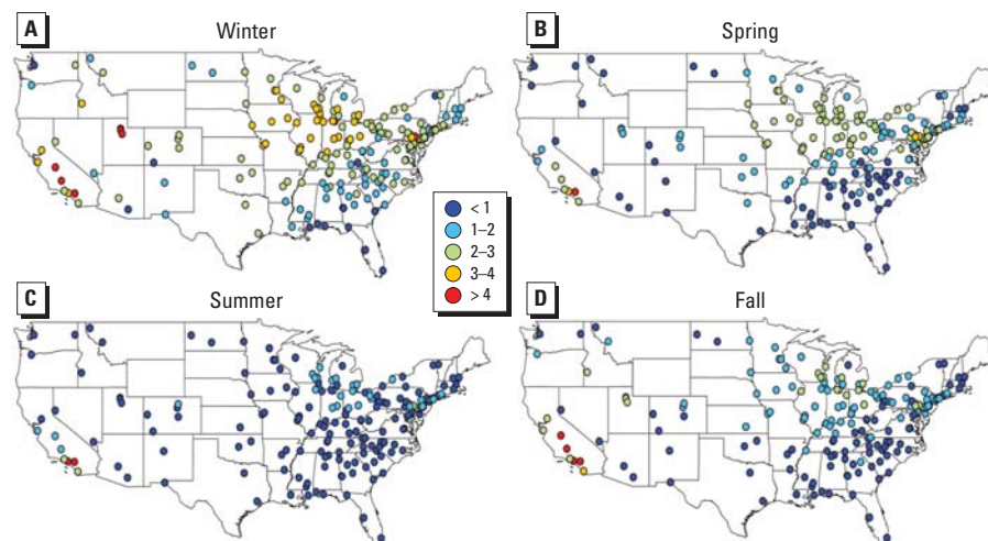
Figure 7. Seasonal nitrate PM 2.5 averages ( \mu\text{g}/\text{m}^3 ) for 187 U.S. counties, 2000–2005.
