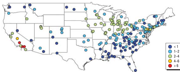
Figure 6. Nitrate PM 2.5 averages ( \mu\text{g}/\text{m}^3 ) for 187 U.S. counties, 2000–2005.
